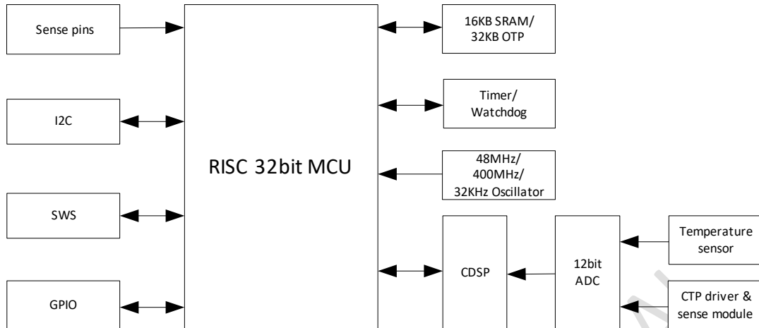
Figure 2- 1 Block diagram
