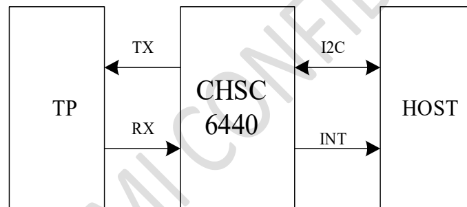
Figure 6- 1 Schematic diagram for interface
