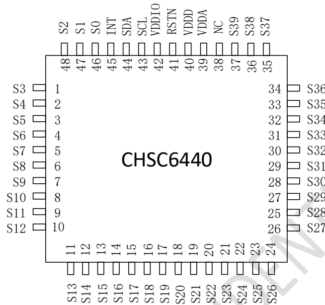
Figure 1- 2 Pin assignment for the CHSC6440
