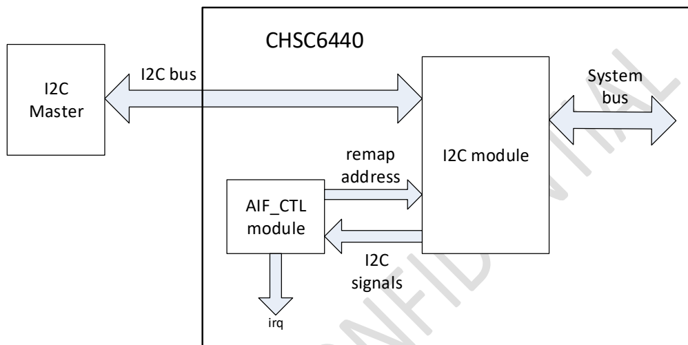
Figure 6- 2 Connection schematic between I2C and AIF_CTL module
