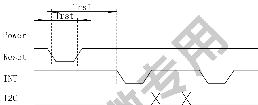
Figure 3-8 Reset Sequence
