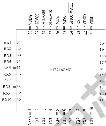
FT5216GM7 Package Diagram
